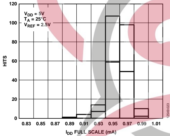
Figure 20. I_{DD} Histogram with External Reference
