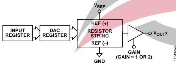
Figure 41. Single DAC Channel Architecture Block Diagram
